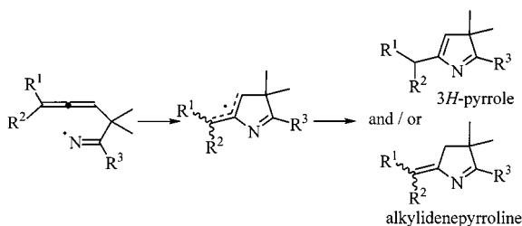
Scheme 1. Reaction of \beta -allenyliminyl radicals
